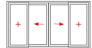
Four part element with two sliding doors in the centre and one fixed pane on each side
