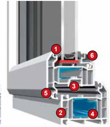
Chamfered C70 System.
